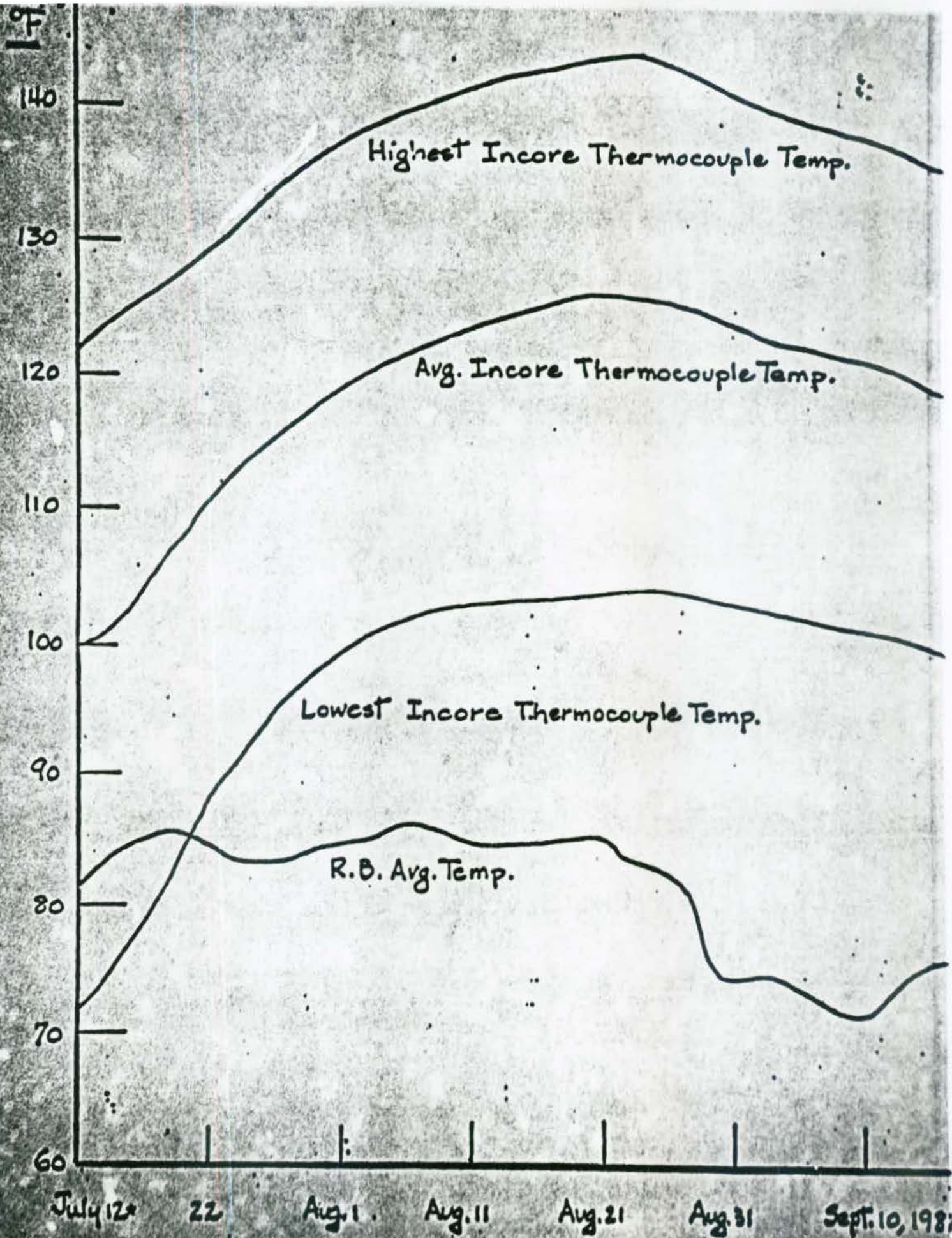
FIGURE 1 - REACTOR BUILDING AND INCORE THERMOCOUPLE TEMPERATURES
